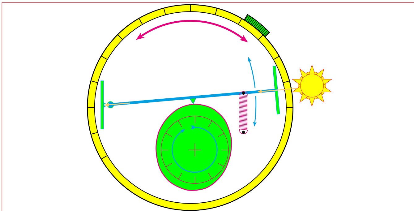
Pillinton Gibbs' mechanism. The precision-made green cam is attached to the circular bronze date-adjustment (see previous illustration).
