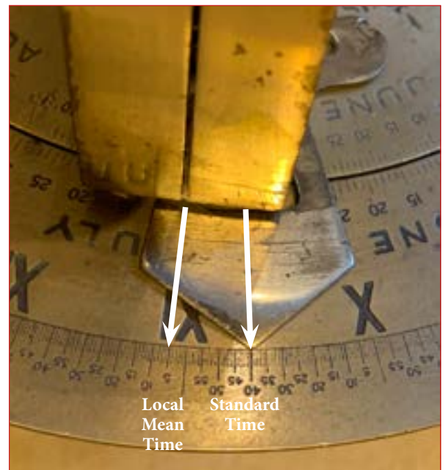
Sol Horometer. The bronze arrow is set for the Longitudinal offset, allowing both local mean time and standard time to be read.
