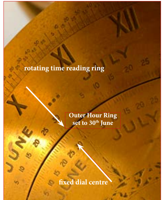
Sol Horometer - EoT alignment scales. Notice the scales for one month is separated from those of the next month to provide clarity. 'Equation of Time Nomograms' on page 103, where a similar technique is used.
