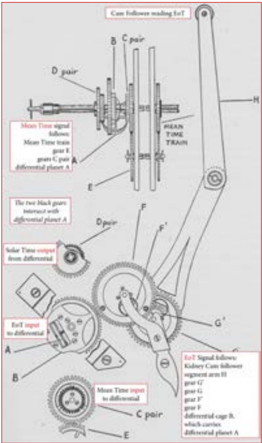
Details of the Differential Adder.
