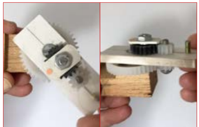
Goodman's Tusi method without a ring gear. On rotation, the orange spot moves linearly with sinusoidal motion
