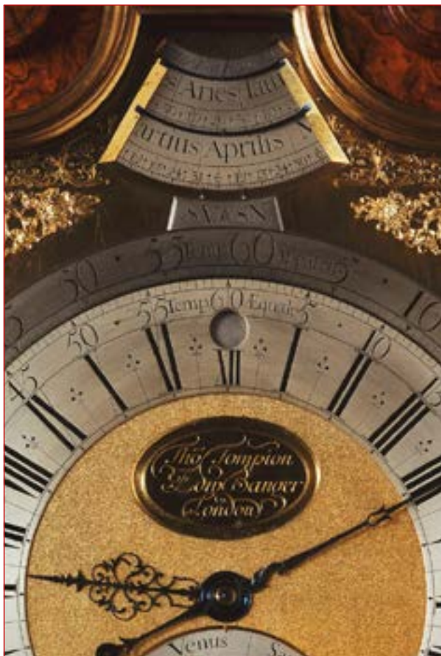
Detail of Tompion & Banger - 1703. Note the Date scale reads 2nd April Julian (SV) and 13th April Gregorian (SN). On this day, the clock gives an EoT of -1 min 20 secs. Tompion's own table (see page 91) for this date in 1683 gives an EoT of 2 mins 4 secs
