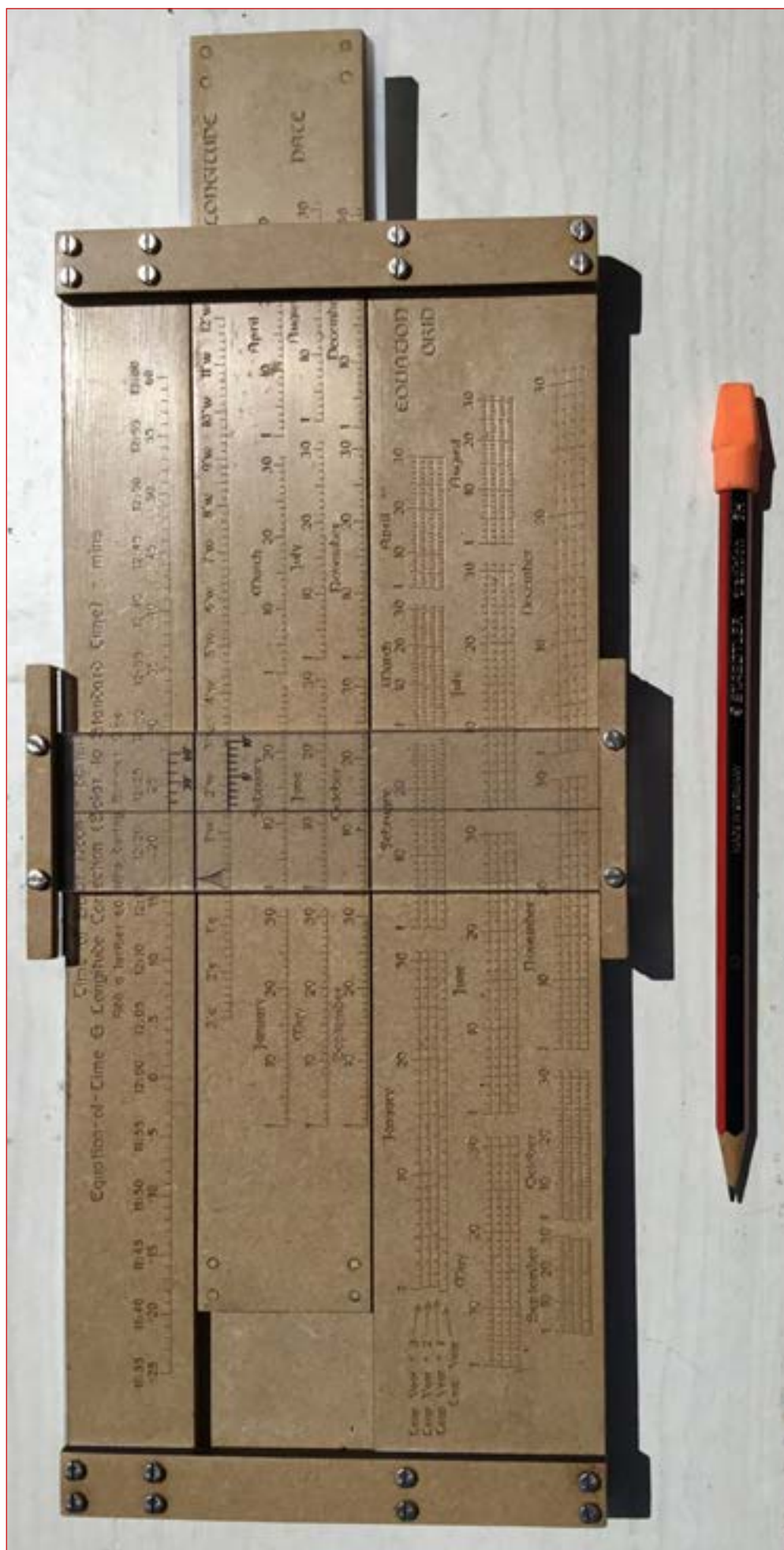
The Gnomonic Instrument Gnomonic (GIN).- as made for the British Isles
