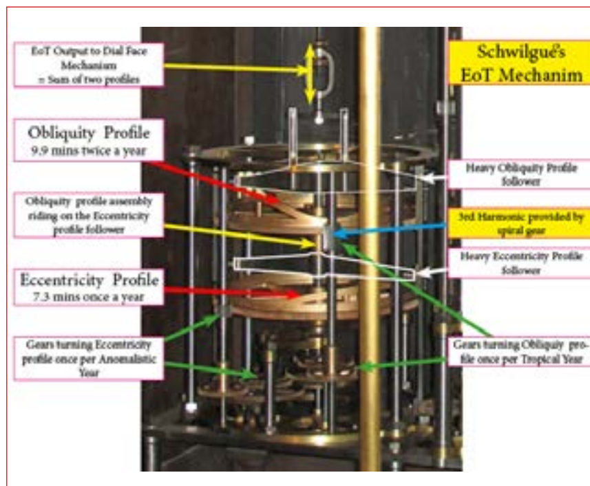
Schwilgué's EoT Mechanism in Detail
