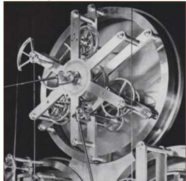
Detail of Rear of Equation Face : Whole works - top left is the quarter-round sector with steel ribbon from Equation mechanism and to left centre, the connection rod to main pendulum mean time mechanism
