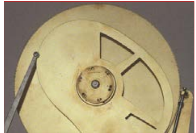
Equation Mechanism from Front
