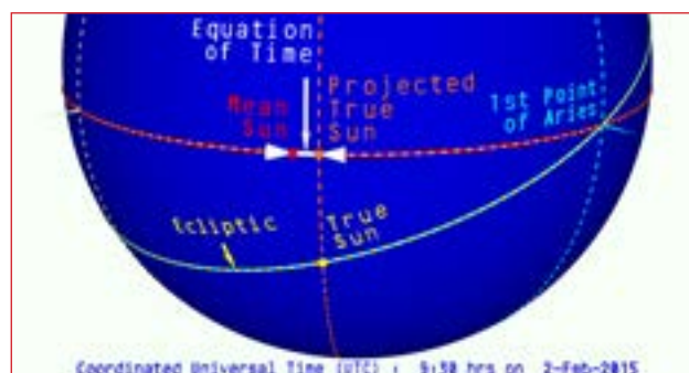
Fig. 7. The Equation-of-Time
