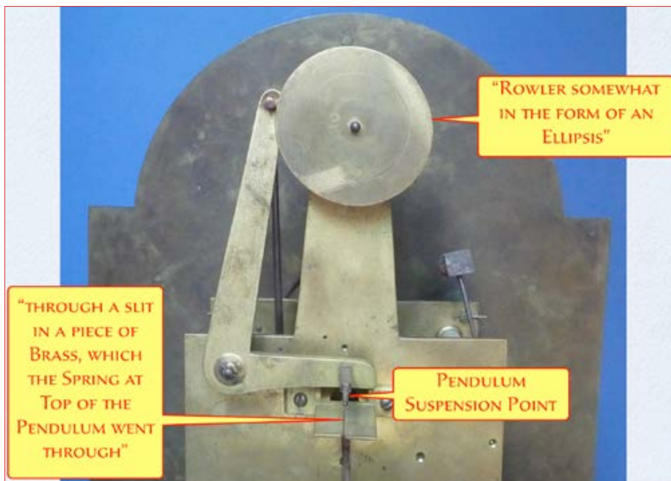
Willamson's Variable Length Pendulum Mechanism
