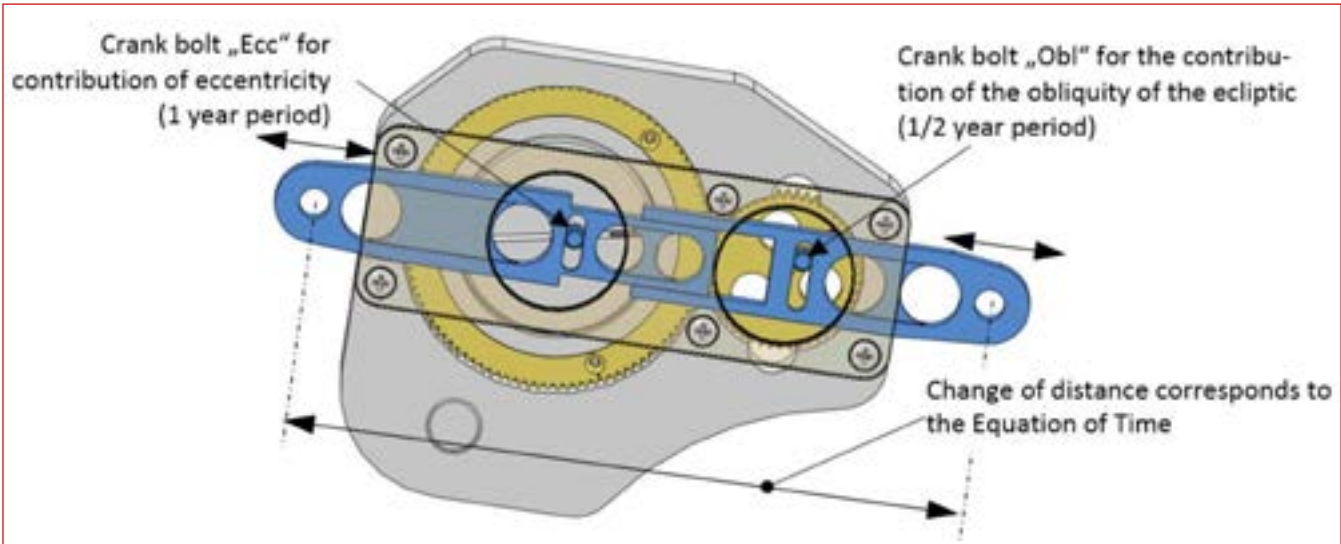
The Equation Mechanism See also 'Descovitch Method' on page 113.
