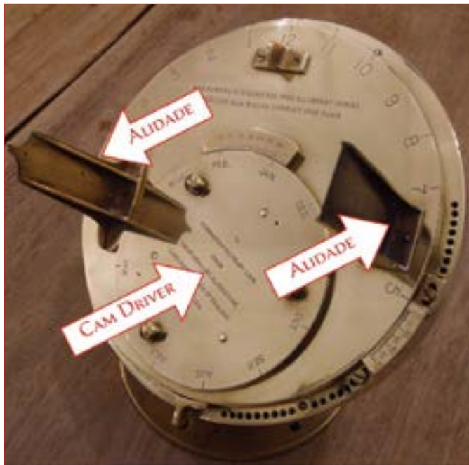
the mechanical working of a Pilkington Gibbs - showing the cam and its follower, which is attached to the alidade .
