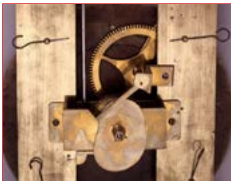
The vertical shaft comes from above driven by the main clock mechanism giving the Date directly and the Equation of Time via the kidney cam.
